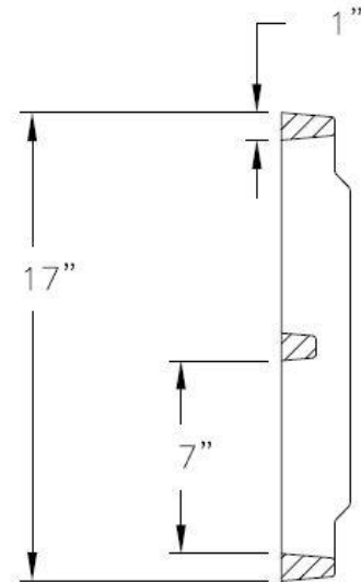
GRATE SECTION
