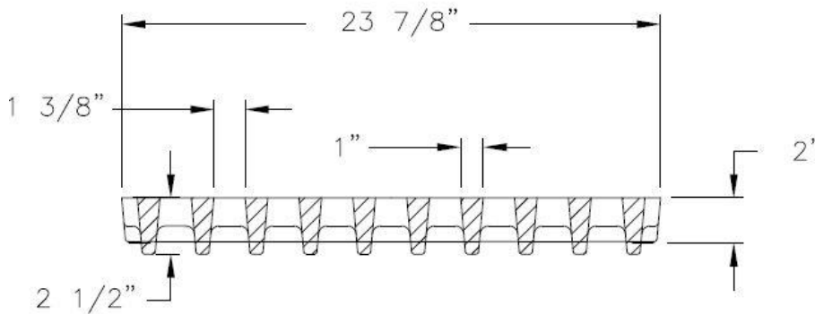
GRATE SECTION
